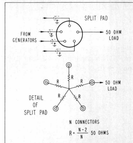
Fig. 3. Method for combining 212A's to obtain best rise time.
