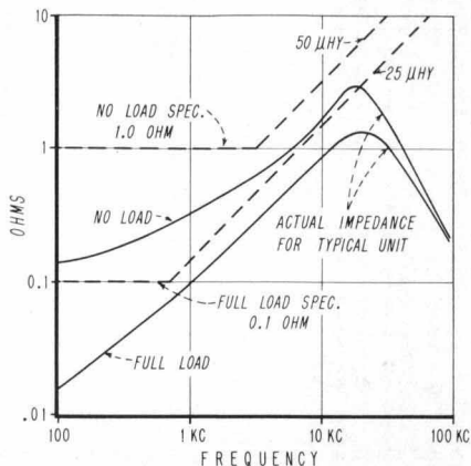
Fig. 4. Impedance characteristics of main output of typical 712B power supply under load and no-load conditions. Rated impedance is shown in dashed lines.
