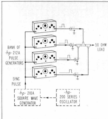
Fig. 1. Method for combining bank of -hp- 212A Pulse Generators to obtain high output pulse trains. Up to 10 generators can be used to provide peak pulse voltages of 30 volts.
