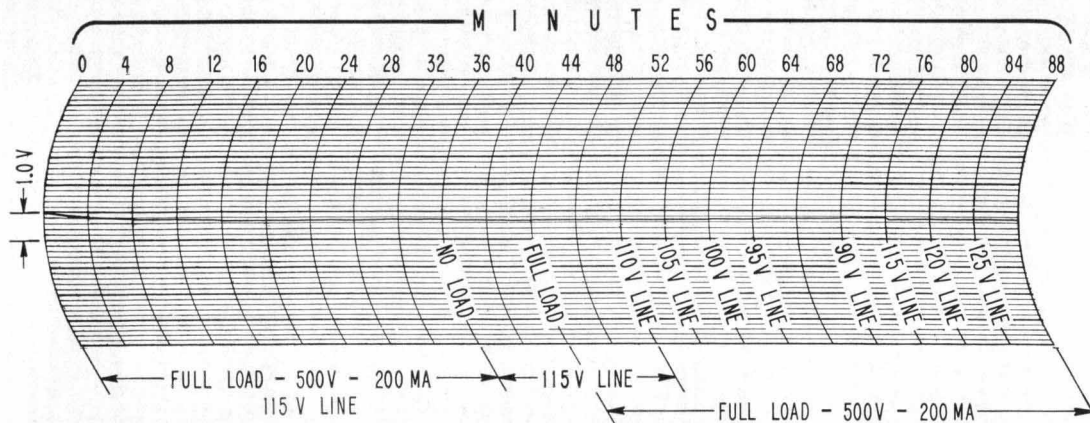
Fig. 2. Record made of main output voltage while 712B was subjected to wide changes in line voltage and output current.
