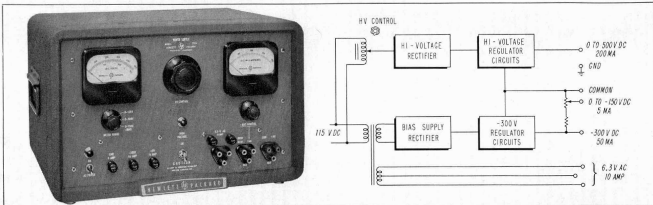
Fig. 1. New -hp- Model 712B Regulated Power Supply provides up to 100 watts of plate power as well as bias and filament supplies. Diagram at right indicates terminal arrangement and ratings of various outputs.
