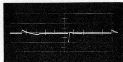
Fig. 3. Transient response of main output. First transient corresponds to change from full current to no current. Notch at center corresponds to change from no current to full current. Amplitude of large notch is only 0.2 volt and dies out in 25 microseconds.
